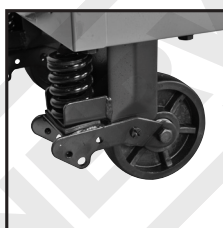
Fixed Wheels (x2)
